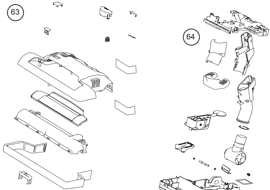
Power Nozzle Upper Assembly
